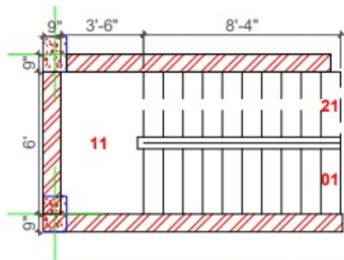
TYPICAL STAIRCASE PLAN
