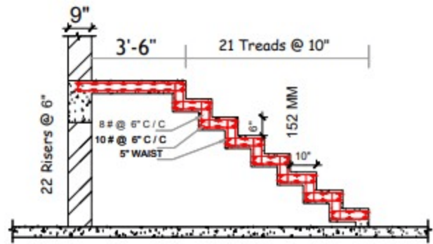
STAIRCASE RCC DETAIL FLOOR HEIGHT 10'-6"
