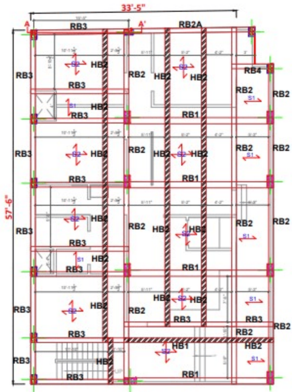
GF ROOF BEAM & SLAB PLAN
