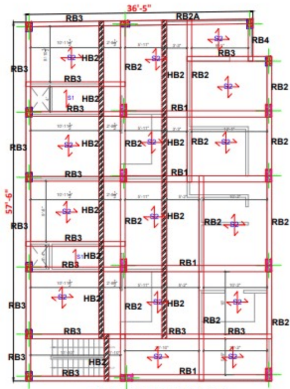
FF ROOF BEAM & SLAB PLAN
