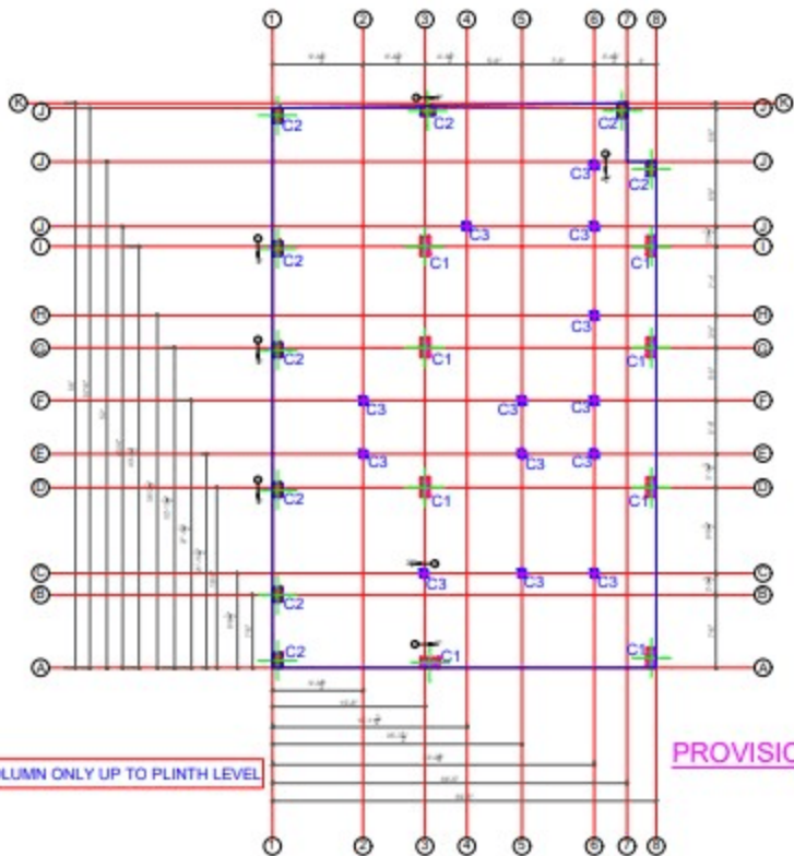
ROAD COLUMN CENTERLINE PLAN
