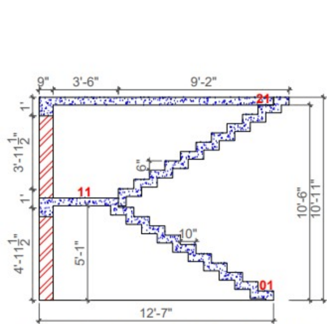
TYPICAL STAIRCASE SECTION
